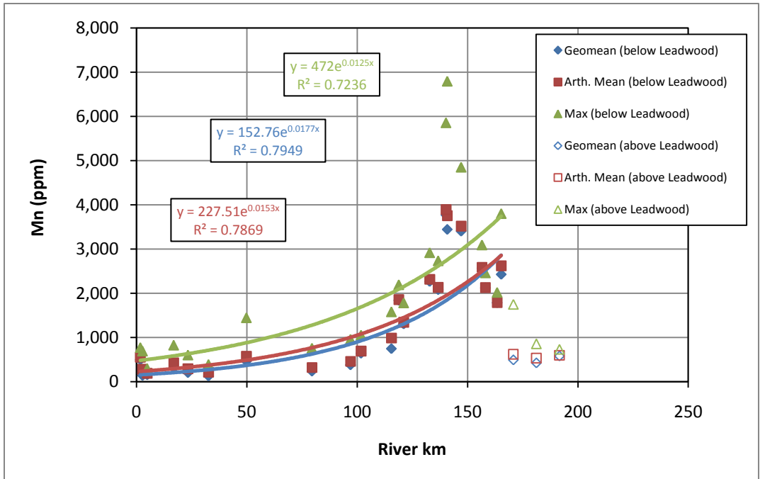
Figure 12C: Downstream Trends Channel Sediment Mn
