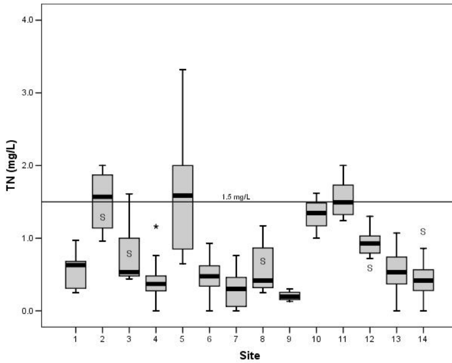
Figure 5. Total Nitrogen (TN) Data by Sample Site
