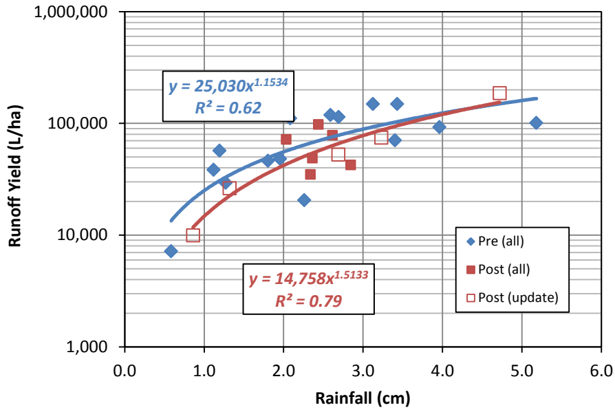
Figure 5. Rainfall-runoff relationship for Drury IN
