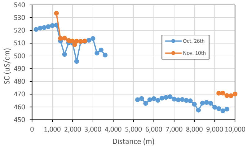
Figure 4. Downstream water parameter trends.
