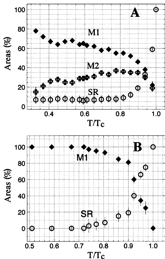
FIG. 3. The abundances (areas) of small spin clusters SR (with superparamagnetically relaxed peaks), and ferromagnetic phases ( M1 ) and ( M2 ) as a function of T/T_c for \text{La}_{0.7}\text{Ca}_{0.3}\text{Mn}^{(57)\text{Co}}\text{O}_3 (A) and \text{La}_{0.8}\text{Ca}_{0.2}\text{Mn}^{(57)\text{Co}}\text{O}_3 (B).
