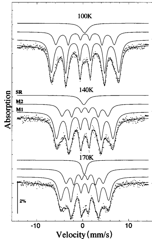
FIG. 2. Computer analyzed Mössbauer spectra of \text{La}_{0.7}\text{Ca}_{0.3}\text{Mn}^{(57\text{Co})}\text{O}_3 at some intermediate temperatures showing two distinct electronic phases designated as M1 and M2 .
