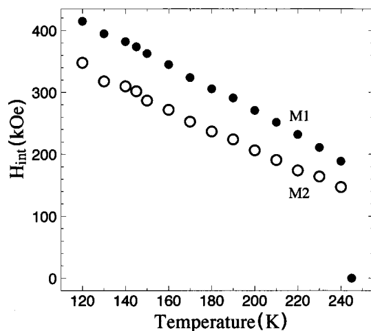
FIG. 4. The plot of internal hyperfine fields H_{\text{int}} at ^{57}\text{Fe} nuclei for the two ferromagnetic phases M1 and M2 in \text{La}_{0.7}\text{Ca}_{0.3}\text{Mn}^{(57)\text{Co}}\text{O}_3 as a function of temperature.
