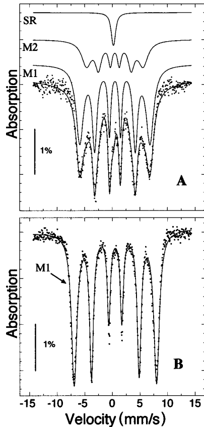
FIG. 1. Computer analyzed Mössbauer spectra of \text{La}_{0.7}\text{Ca}_{0.3}\text{Mn}^{(57\text{Co})}\text{O}_3 with T_c = 245 K (A) and \text{La}_{0.8}\text{Ca}_{0.2}\text{Mn}^{(57\text{Co})}\text{O}_3 with T_c = 195 K (B) at 78 K.
