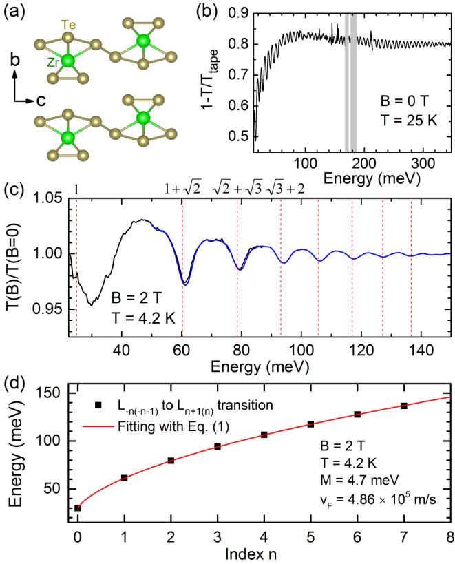
FIG. 1. (a) Schematic view of \text{ZrTe}_5 unit cell along the a axis. The layer stacking direction is along the b axis. (b) Extinction spectrum, 1 - T/T_{\text{tape}} , of \text{ZrTe}_5/\text{tape} composite measured at B = 0 T and T = 25 K. The fast oscillations originate from the Fabry-Pérot interference. The gray stripes cover the opaque regions due to tape absorption. (c) Normalized transmission spectrum, T(B)/T(B=0) , measured at B = 2 T and T = 4.2 K. The black and blue curves correspond to the far-IR and the mid-IR spectrum, respectively. The red dashed lines mark the expected energies of L_{-n(-n-1)} \rightarrow L_{n+1(n)} transitions for massless Dirac fermions. (d) Extracted LL transition energy from (c) as a function of LL index n . The red line shows the best fit to the data using Eq. (1).
