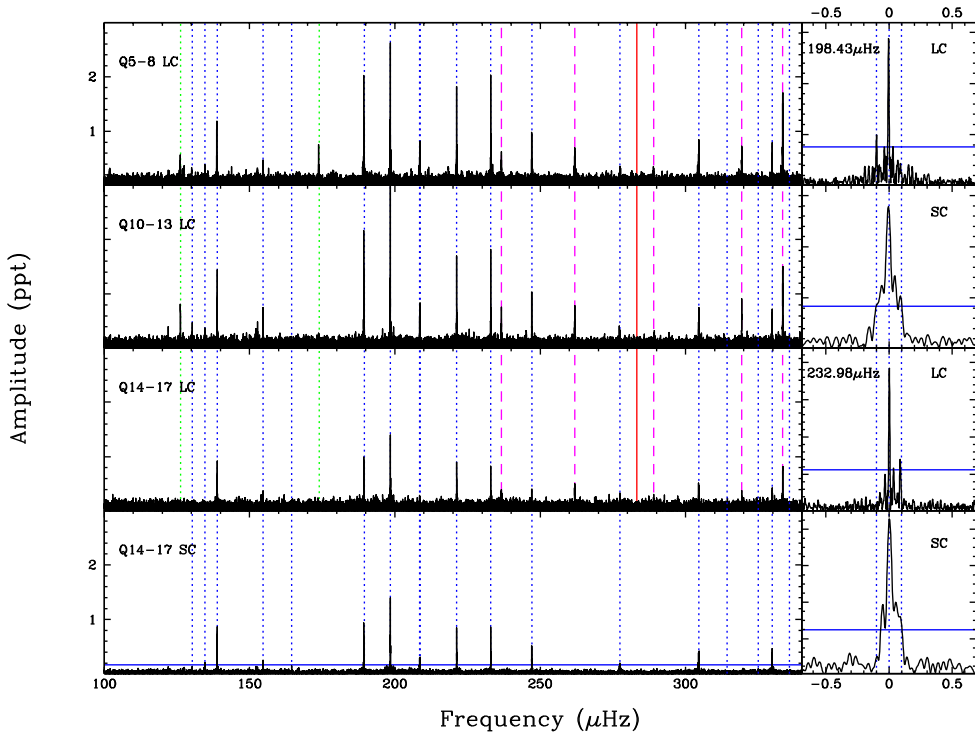
Fig. 1. Amplitude spectra for the sdB star KIC 2569576, located in NGC 6791. The left panels show different segments of long cadence (LC) data from the superstamps (top three panels) compared to the short cadence (SC) data obtained through GO observations (bottom panel). The green lines indicate frequencies that were not seen during the SC observing period but which are evident in the other quarters. The right panels show two multiplets in both SC and LC data; the full 17 quarters of LC data from the superstamps allow the multiplets to be resolved which was not possible with only the SC data from quarters 14-17 from GO observations.
