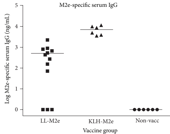
FIGURE 3: Serum response. Serum was collected 1 week after final vaccination and analyzed for M2e-specific serum IgG by ELISA using microtiter plates coated with 2 \mu\text{g/mL} M2e peptide. The plates were developed with goat antichickens IgG-horseradish peroxidase conjugate and chemiluminescent substrate. Luminescent signal from each sample was converted to concentration of chicken IgG by extrapolation from the graph of luminescence versus IgG concentration of the standards and corrected for sample dilution. Each sample was analyzed at two or three different dilutions, and each dilution was analyzed in duplicate. Group mean M2e-specific IgG concentration is shown.
