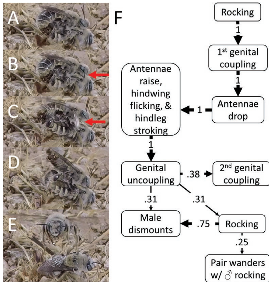
Fig. 1. (a–d) Phases in mating: (a) genital coupling, (b) antennae dropping and contacting the female indicated with the red arrow, (c) antennae raised and hindwing flicking (indicated with the red arrow), (d) genital uncoupling, and (e) male dismounts and male and female fly away. (f) Ethogram of the male mating behavior. Arrows indicate the transition from one behavioral component to another. The transition frequency is indicated by both the number and thickness of the arrow. We calculated values by dividing the average number of transitions for a particular component by the total number of transitions derived from a behavioral element. Thus, transition frequencies reflect only the transitions from a given component to any other component (i.e., all transitions from a given component add up to one). We report data from the averaged response of the full mating sequence for 11 pairs (1 pair dropped after the genital uncoupling component). Photo credit to Bruce Taubert.
