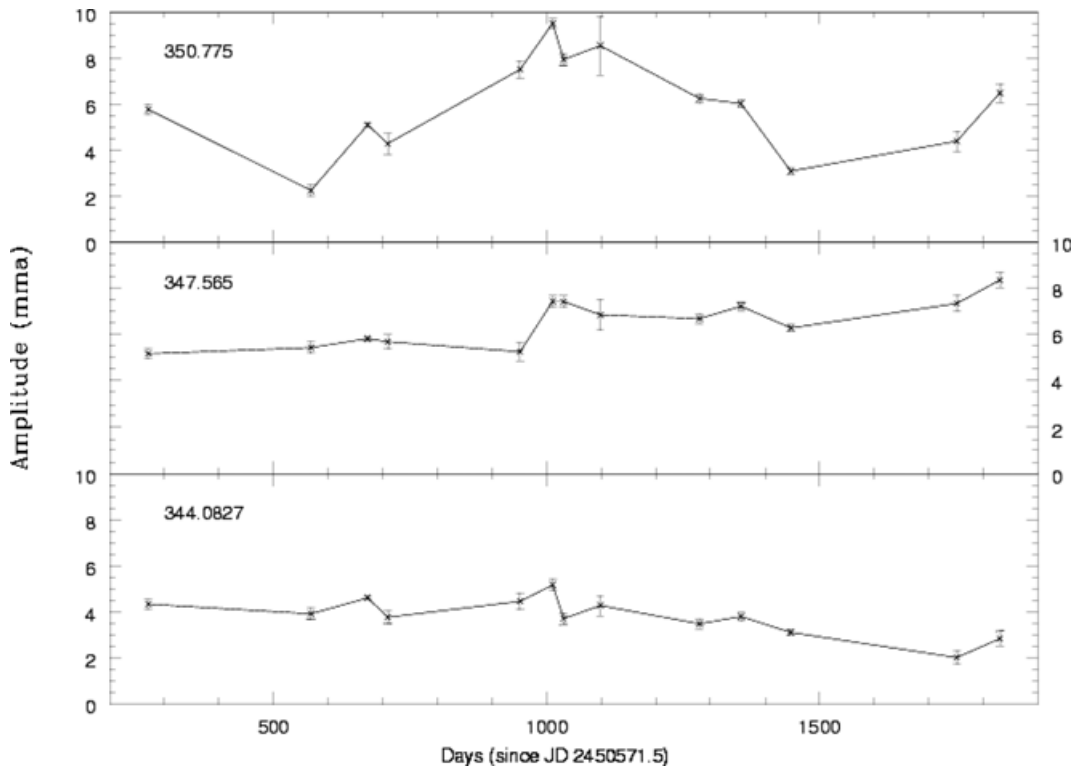
Figure 3. Pulsation amplitudes for the three largest-amplitude modes.
