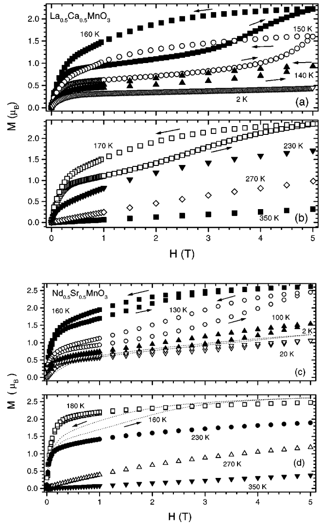
FIG. 2. Magnetization vs applied magnetic field for representative temperatures in \text{La}_{0.5}\text{Ca}_{0.5}\text{MnO}_3 (a) and (b) and \text{Nd}_{0.5}\text{Sr}_{0.5}\text{MnO}_3 (c) and (d) samples. Magnetization is given in Bohr magnetons per manganese ion. The applied magnetic field was cycled in all cases from 0 to 5 T and then back to 0 T again. Ferromagnetic and antiferromagnetic interactions coexist in both compounds, leading to charge and orbital ordered phases.
